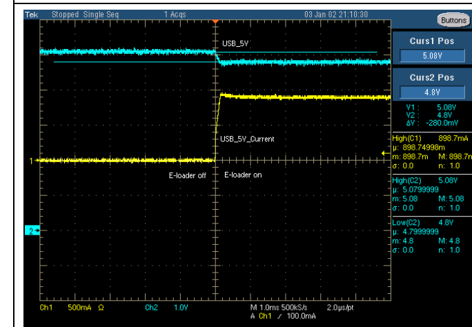
Fig. 3: USB_5V with E-loader [900mA]
